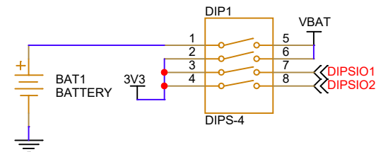
VBAT SWITCH AND ADDITIONAL CONFIG DIP SWITCH
